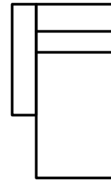
Chaiselongue 98 (G/D) L 98 x P 166 x H 83/100 (assise 75cm)
