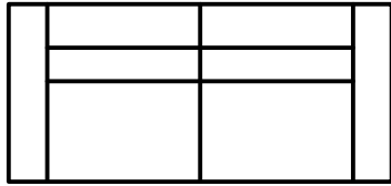
3 Places - 2 assises L 228 x P 106 x H 83/100
