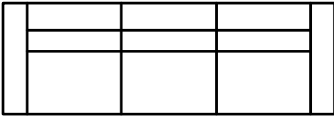
3 Places - 3 assises L 317 x P 106 x H 83/100
