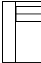
Chaiselongue 108 (G/D) L 108 x P 166/171 x H 95 (assise 70cm)
