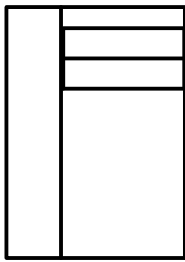
Chaiselongue 118 (G/D) L 118 x P 166/171 x H 95 (assise 80cm)
